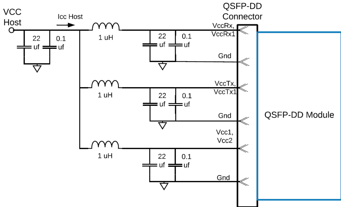
Figure 2 Recommended power supply filter
