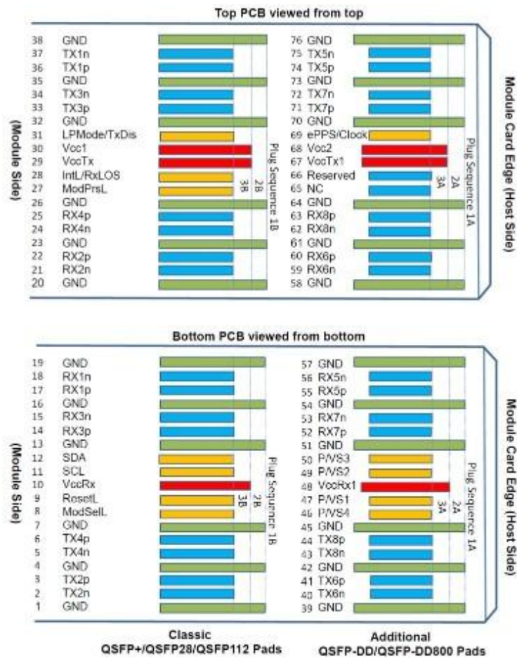
Figure 5 Electrical Pin-out Details
