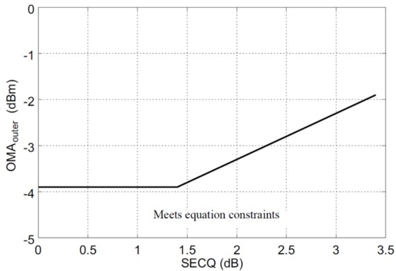
Figure 2 Illustration of Receiver Sensitivity Mask for 800G-DR8
