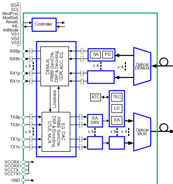
Figure 1 The 400G QSFP-DD FR4 Optical Transceiver Block Diagram
