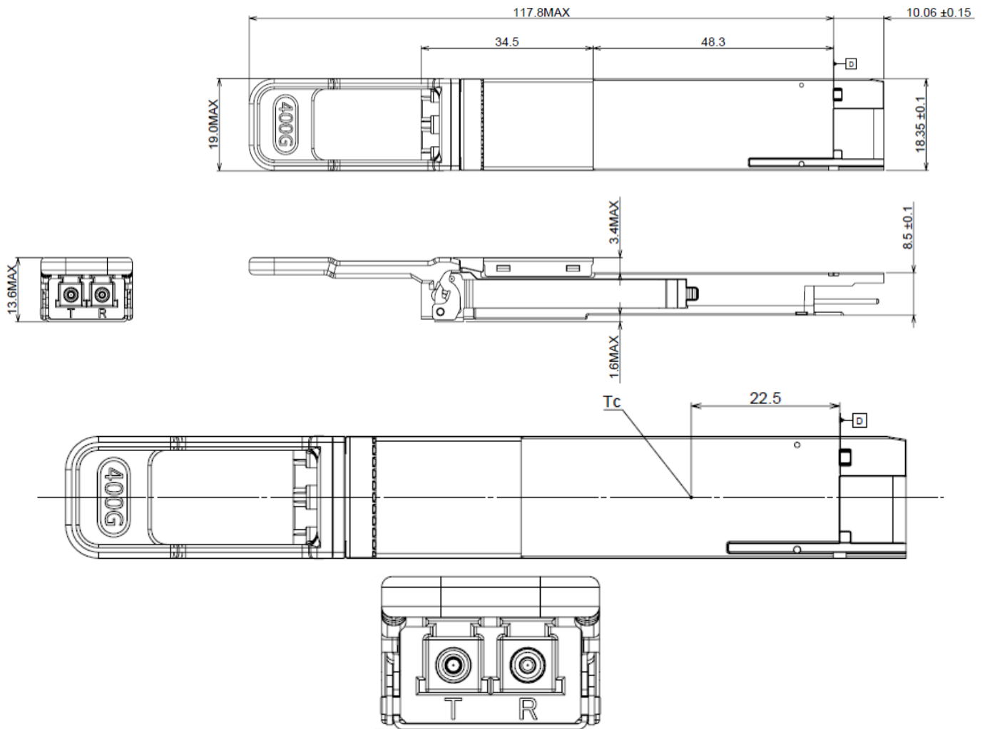
Figure 4 Mechanical Specifications (mm)
