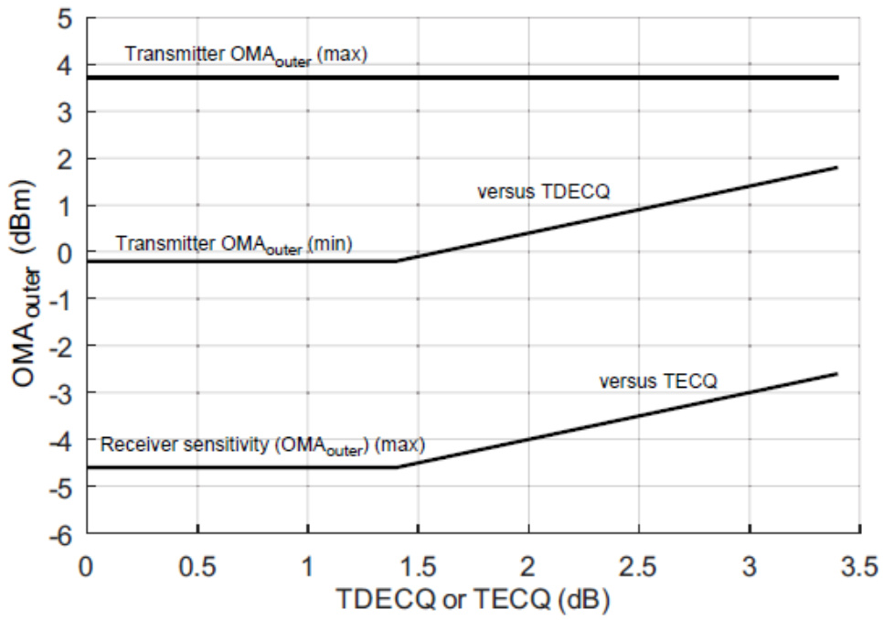
Figure 3 Illustration of Receiver Sensitivity
