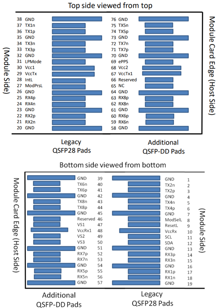
Figure 5 Electrical Pin-out Details
