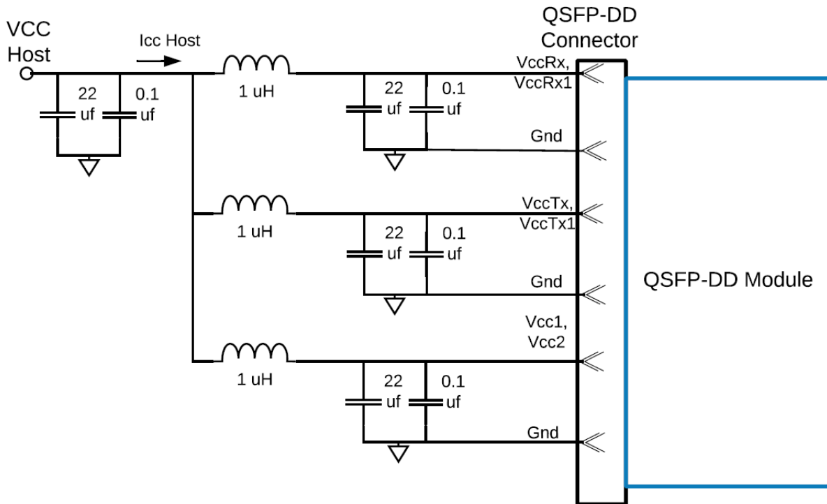
Figure 2 Recommended power supply filter
