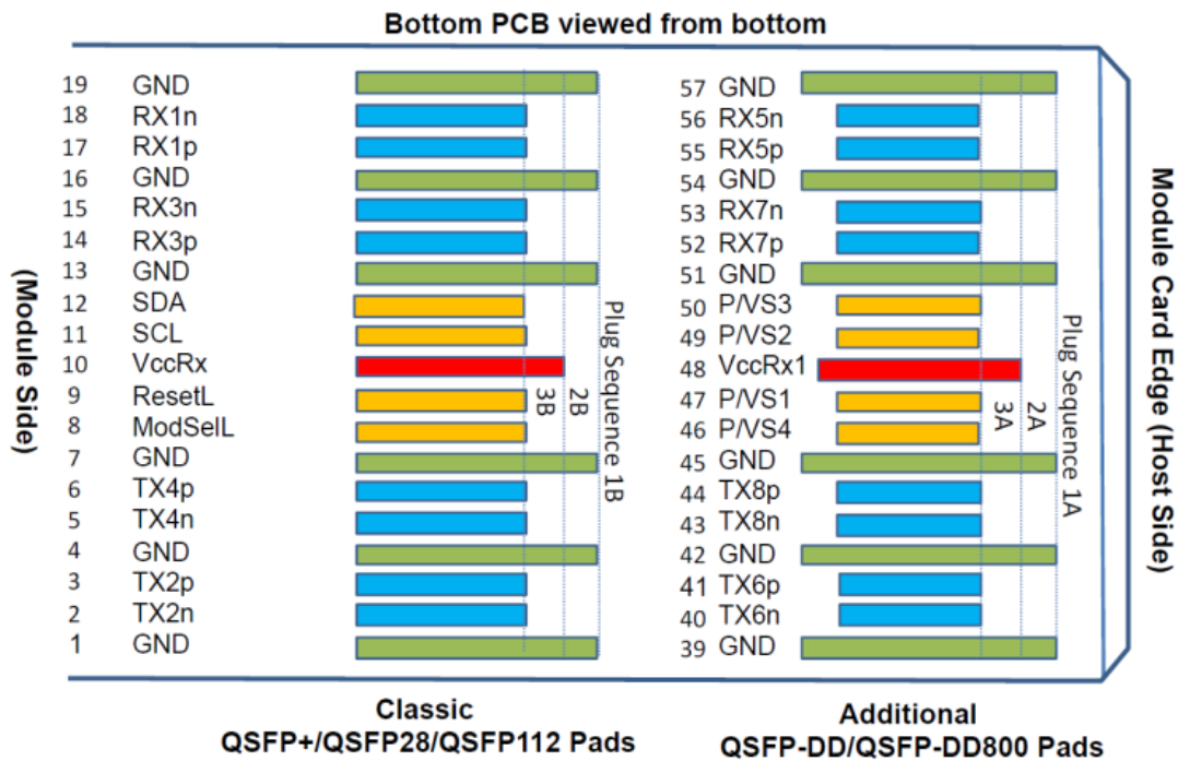
Figure 4 Electrical Pin-out Details
