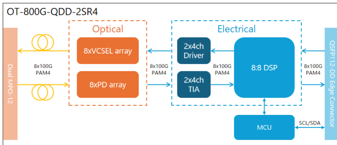
Figure 1 The 800G QSFP-DD 2SR4 Optical Transceiver Block Diagram
