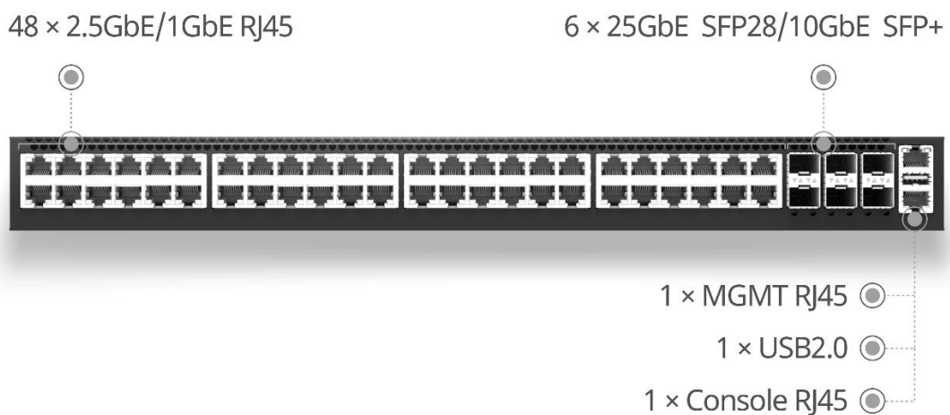
Front panel of CX206Y-48GT/MT-M-H
